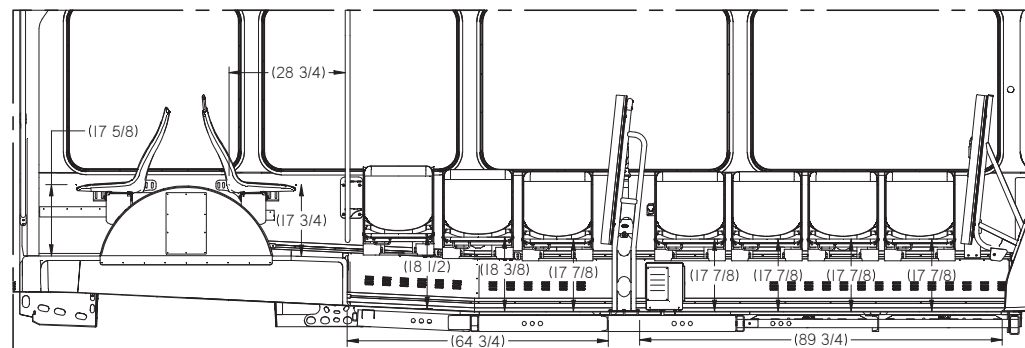
SECTION B: STREET SIDE
