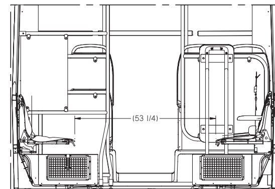
SECTION C: AISLE VIEW
